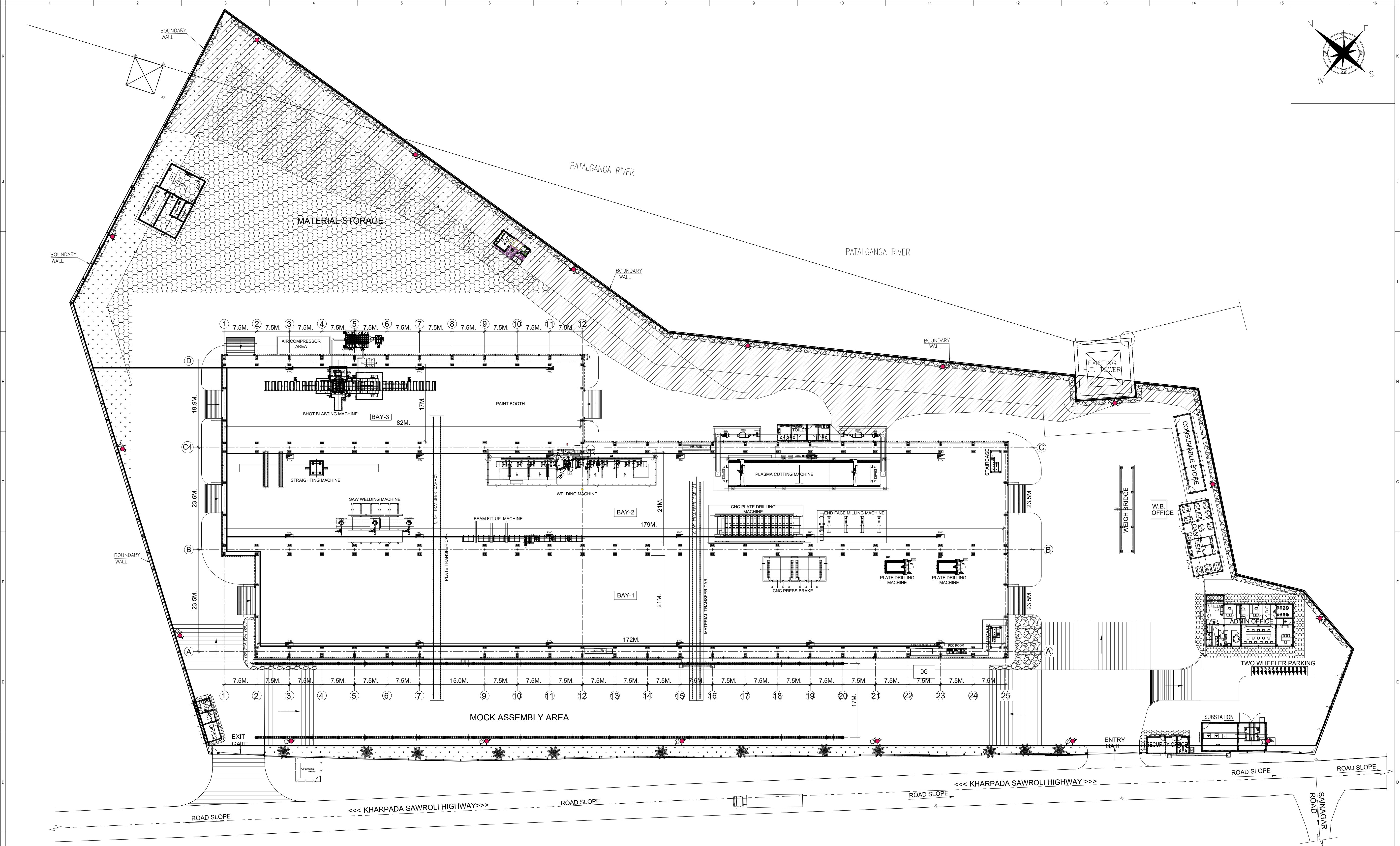
LAYOUT PLAN
